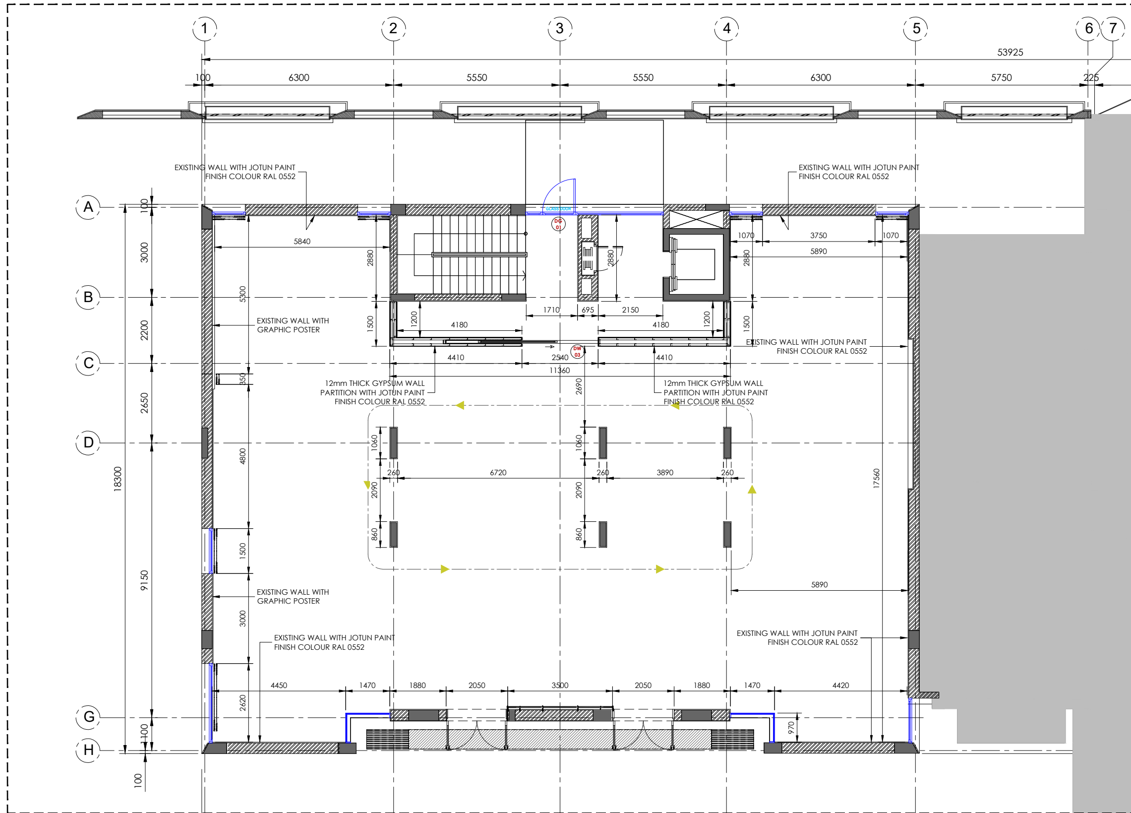
A WALL FINISHES LAYOUT (GF) AR-04 SCALE 1:125
