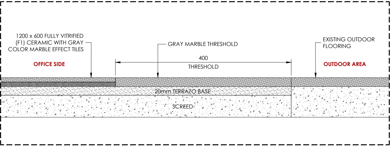
1 AR-03.1 DETAIL SCALE 1:5
