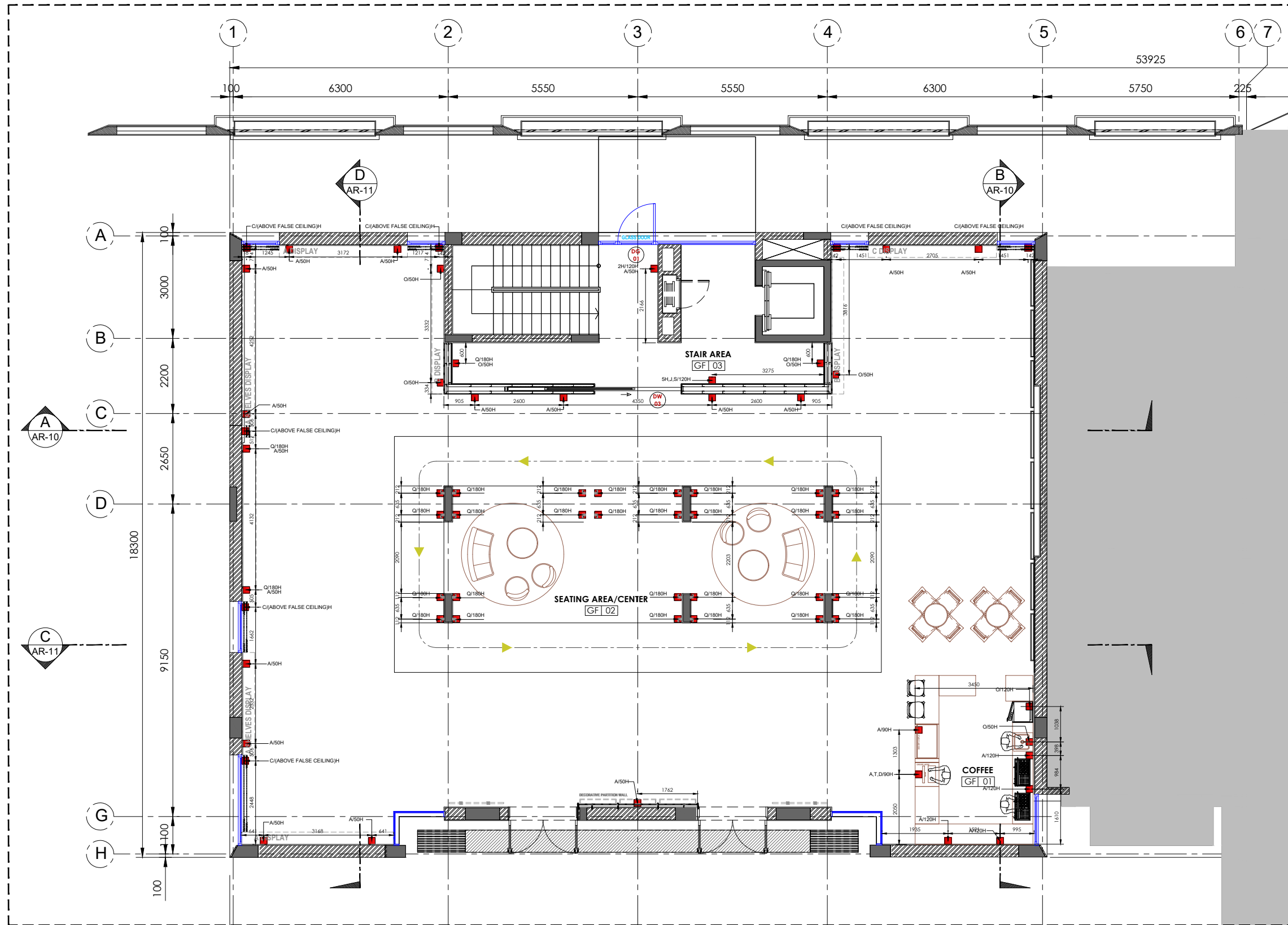
A POWER LAYOUT (GF) EL-02 SCALE 1:125
