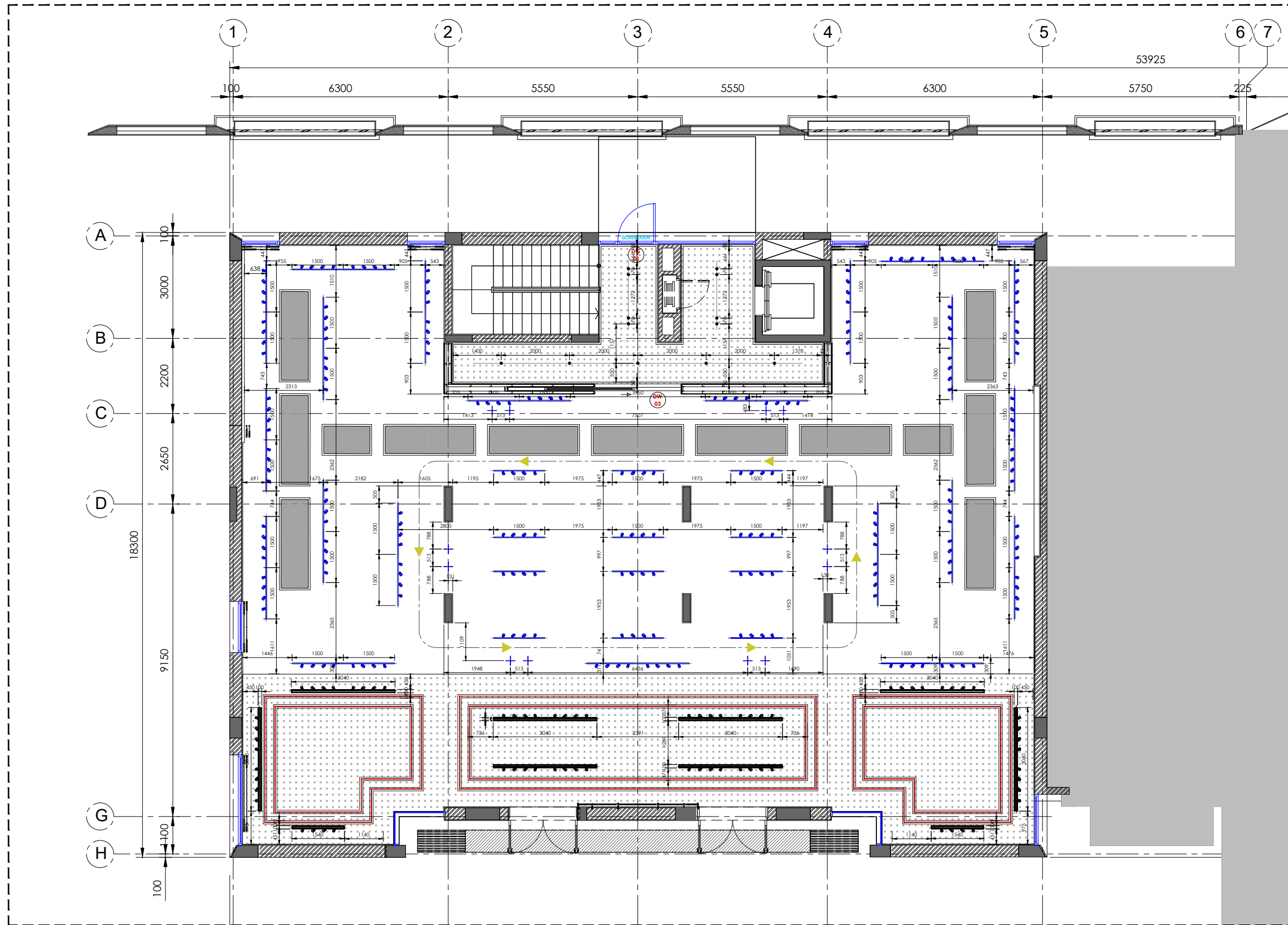
A EL-01 LIGHTING LAYOUT (GF) SCALE 1:125
