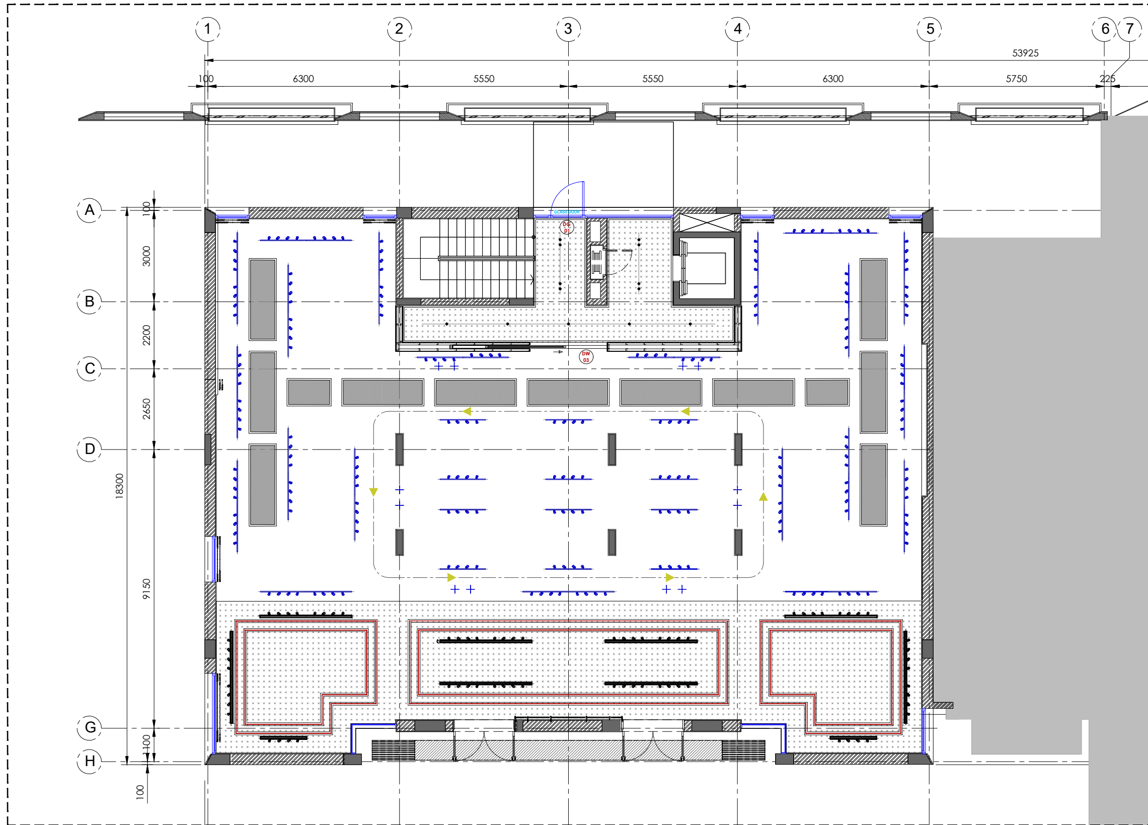
A AR-06 COORDINATED CEILING PLAN (GF) SCALE 1:125
