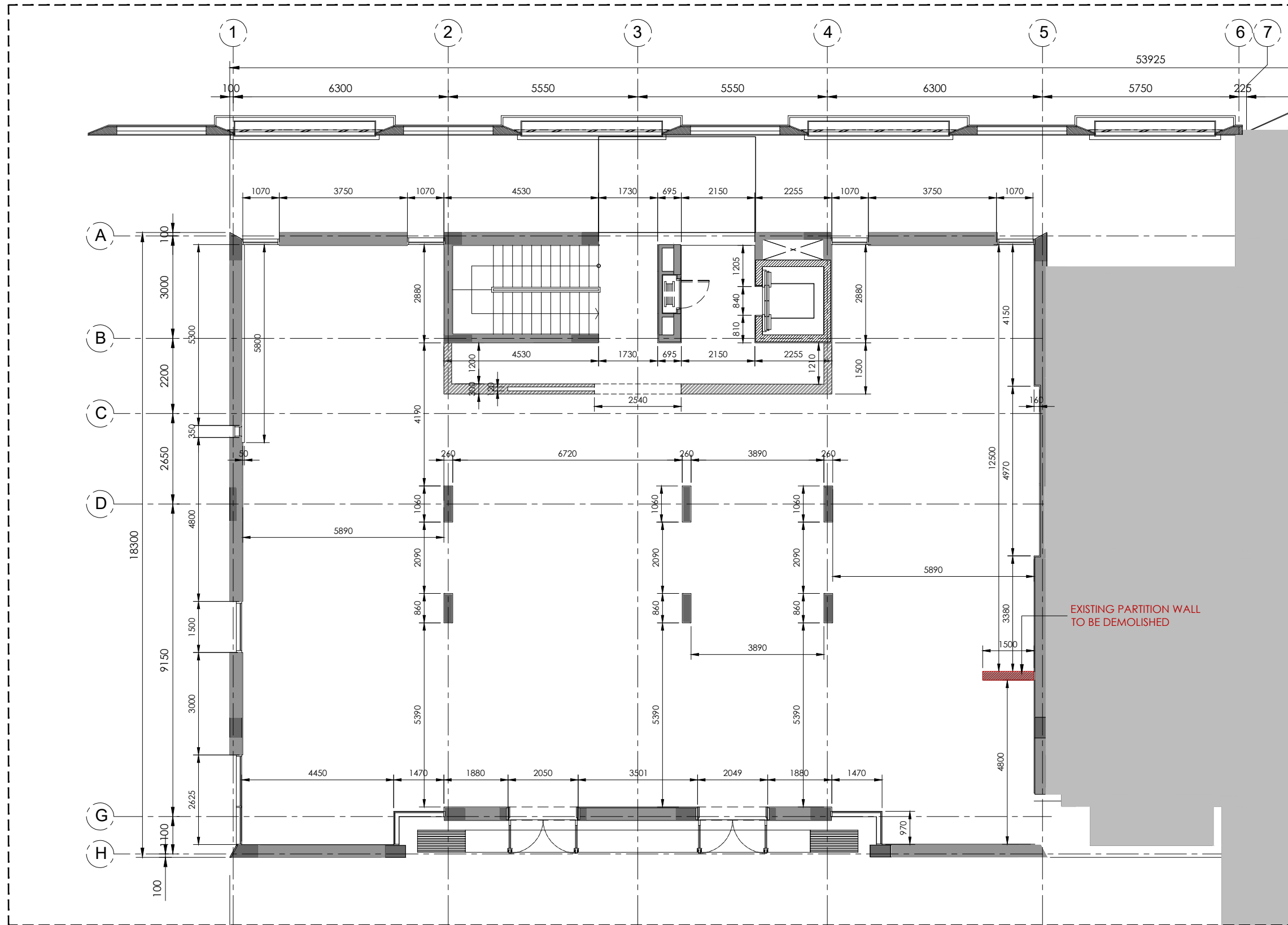
A DEMOLITION LAYOUT (GF) DE-01 SCALE 1:125
