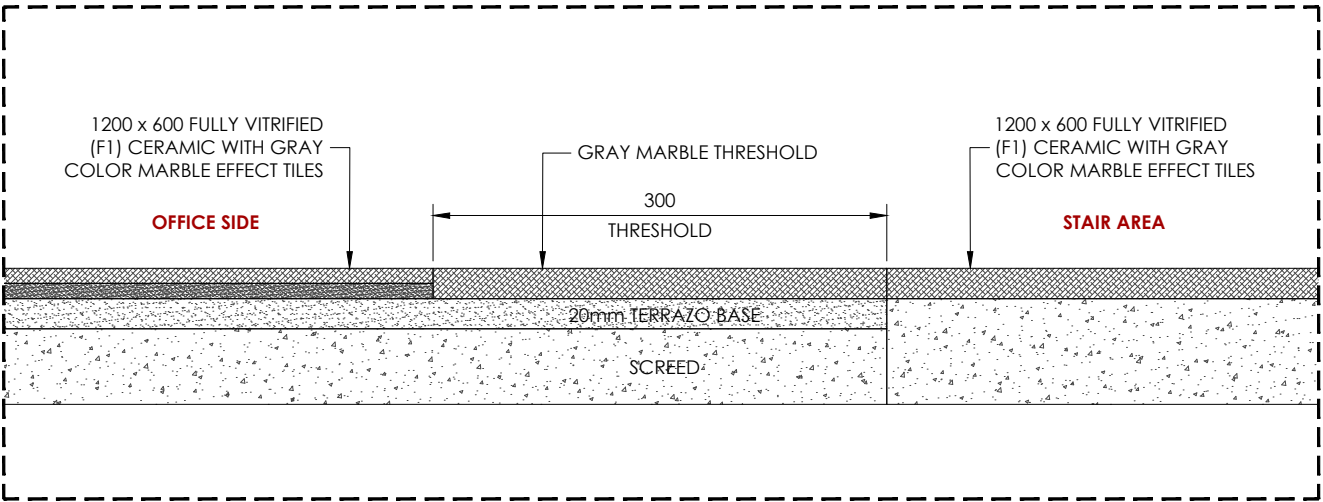
2 AR-03.1 DETAIL SCALE 1:5
