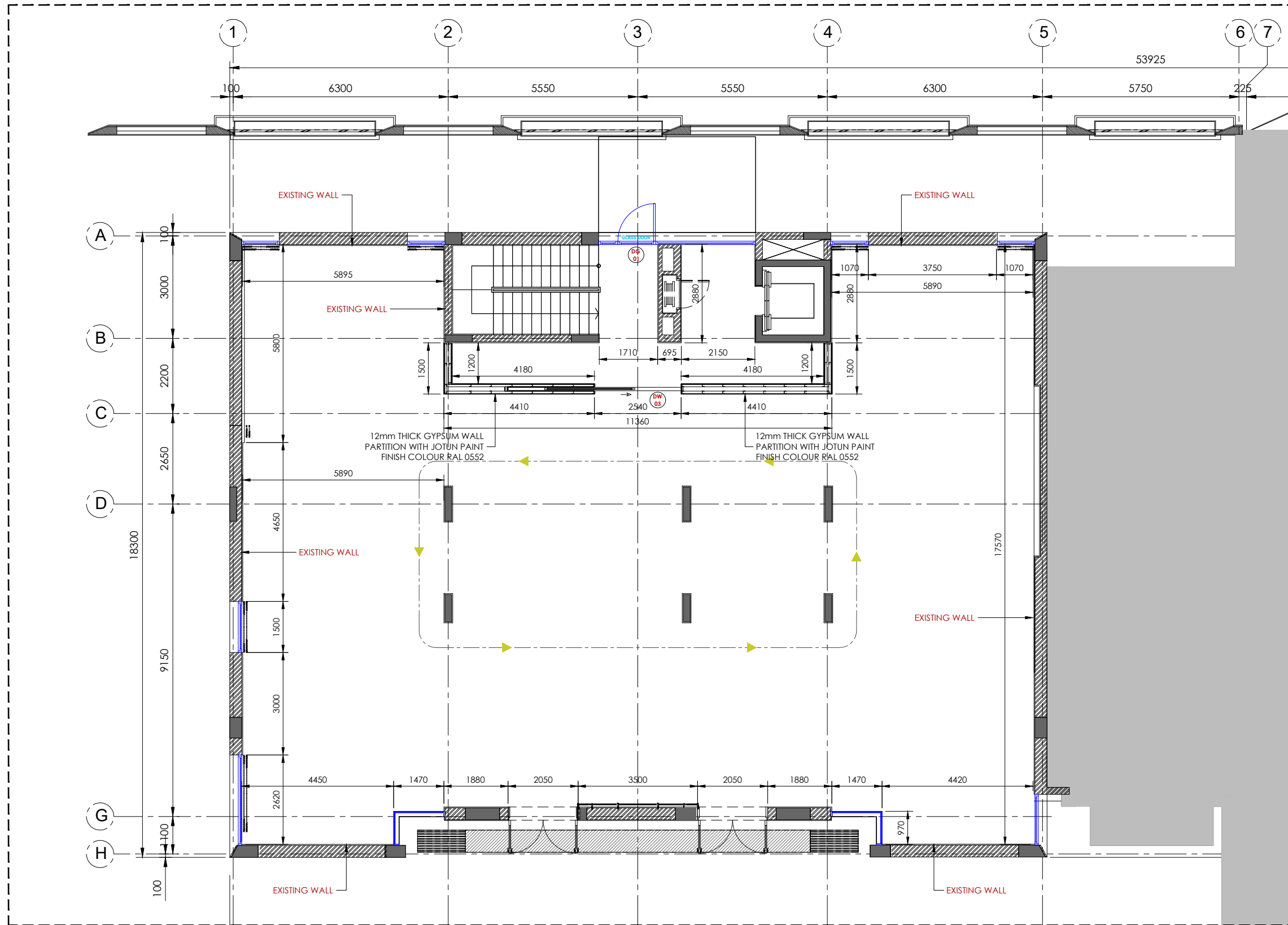
A AR-02 PARTITION LAYOUT (GF) SCALE 1:125
