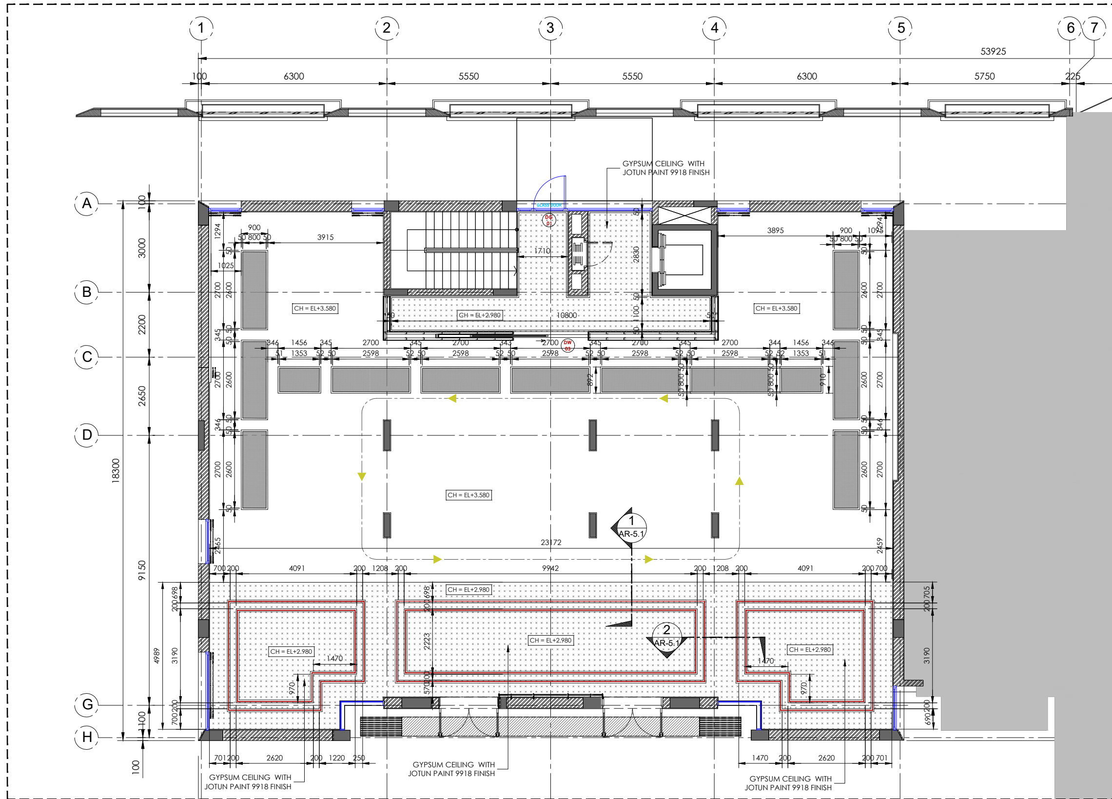
A REFLECTED CEILING PLAN (GF) AR-05 SCALE 1:125
