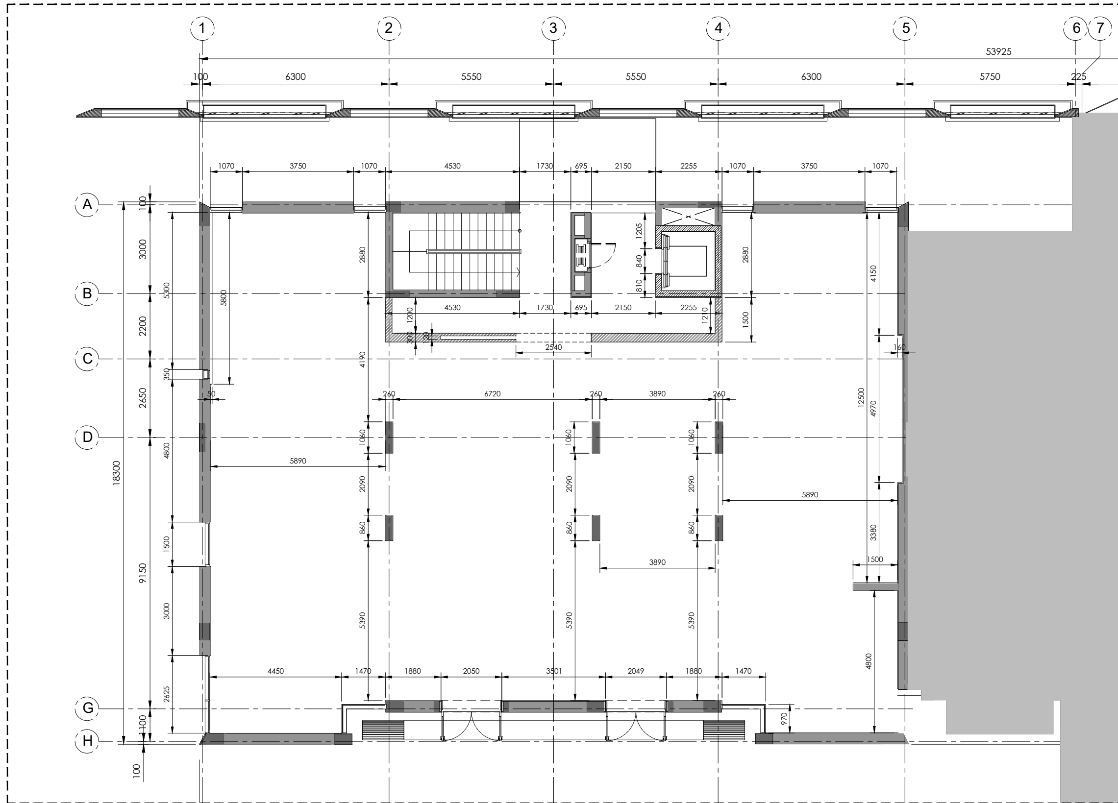
ASBUILT LAYOUT (GF) SCALE 1:125
